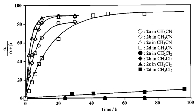
Figure 1. Time dependence of C1' epimerization of 5'-O-acyl-3'-O-toluoylthymidine derivatives 2a–d(β) in acetonitrile and dichloromethane, based on ^1\text{H} NMR analysis; in acetonitrile: open circle 2a(β) , open diamond 2b(β) , open triangle 2c(β) , open square 2d(β) ; in dichloromethane: closed circle 2a(β) , closed diamond 2b(β) , closed triangle 2c(β) , closed square 2d(β)
