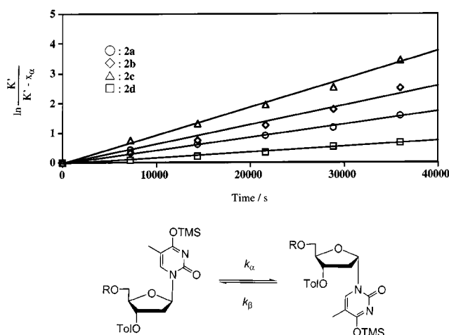
Figure 3. Kinetics of C1' epimerization of 2a–d in acetonitrile
