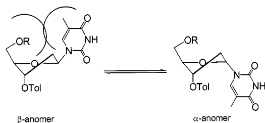
Figure 2. Interaction of the 5'-acyl moiety with the thymine base
